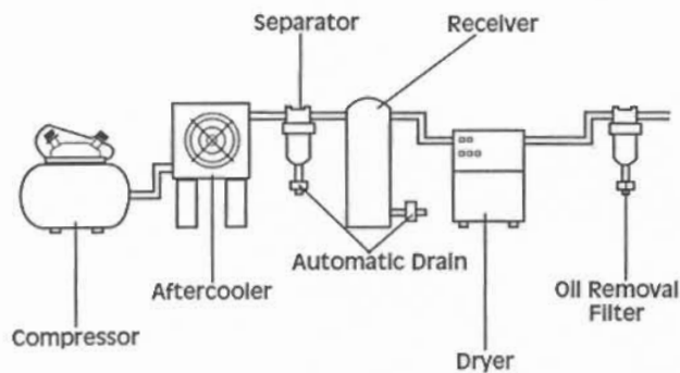
TYPICAL COMPRESSED AIR SYSTEM
